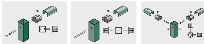
Connection at end post.
